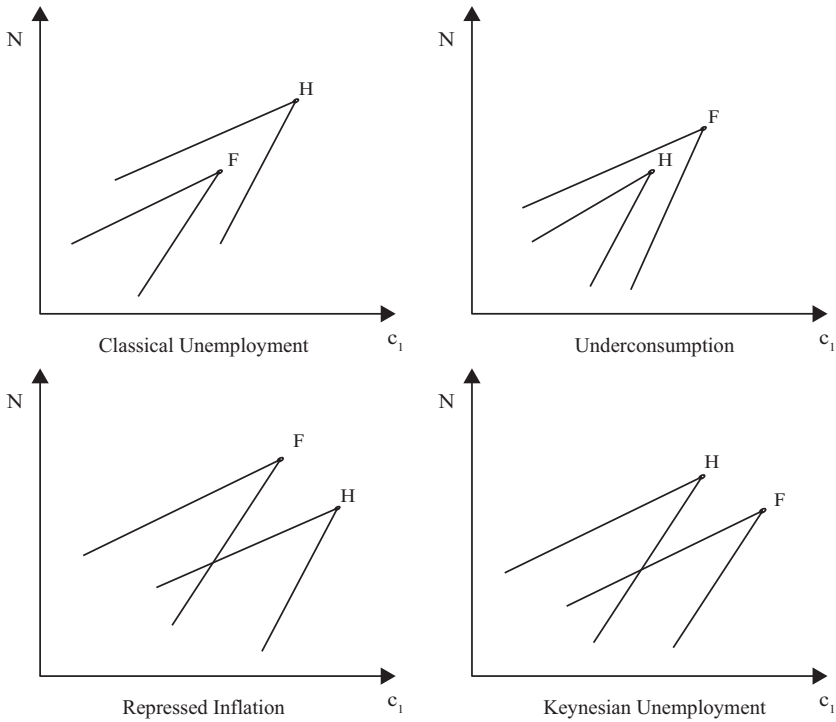
Diagram 5.8 Quantity-constrained regimes
