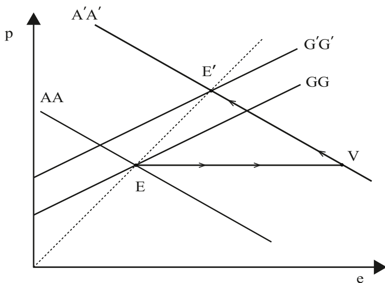
Diagram 12.3 Overshooting
